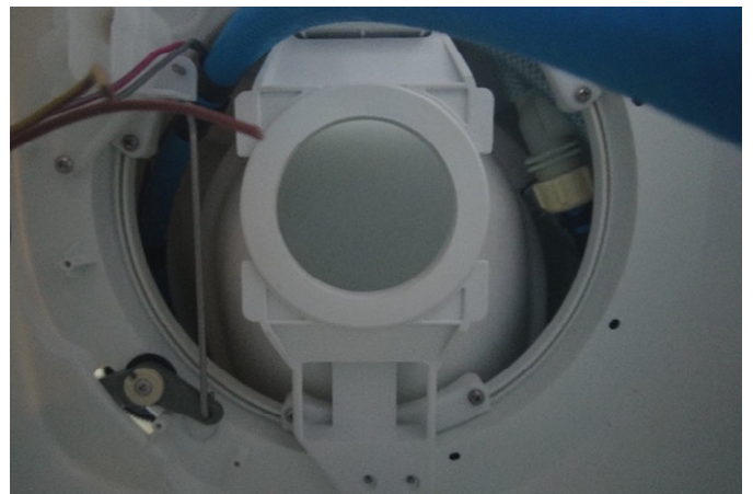
11. Through the service flap, loosen the four screws of the two clamps that secure the seat part of your Thetford chemical toilet to the base. Then pull the clamps off in a clockwise direction.
