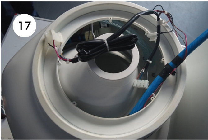
17. Remove the complete bowl with seat part, seat and cover as well as the hose and cable. You will no longer need them. Please keep them for possible dismantling.
