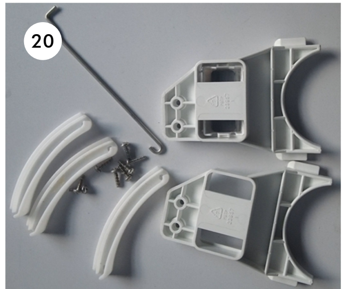
20. You have now removed these parts. The six screws are used to mount the new slide bearings. You will no longer need the remaining parts. Please keep them for possible dismantling.
